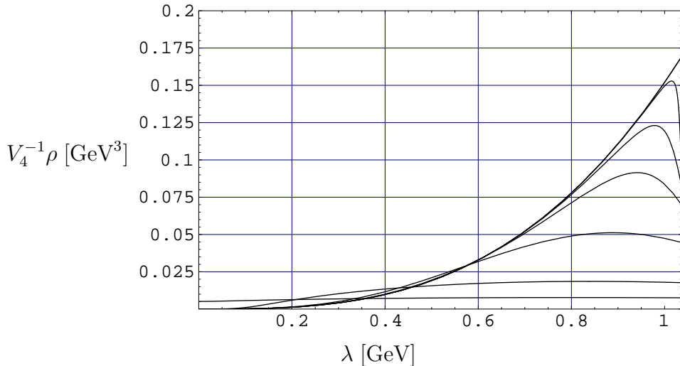
Figure 5: The spectrum for different values of m_\Lambda . As m_\Lambda approaches infinity the curve resembles more and more the free spectrum with a sharp cutoff at \Lambda . The spectra are plotted for m_\Lambda = .228, .5, 1.5, 4, 10, 50, 2000 GeV. The free spectrum differs from the spectrum with m_\Lambda = 2000 only for values of \lambda very close to \Lambda .
